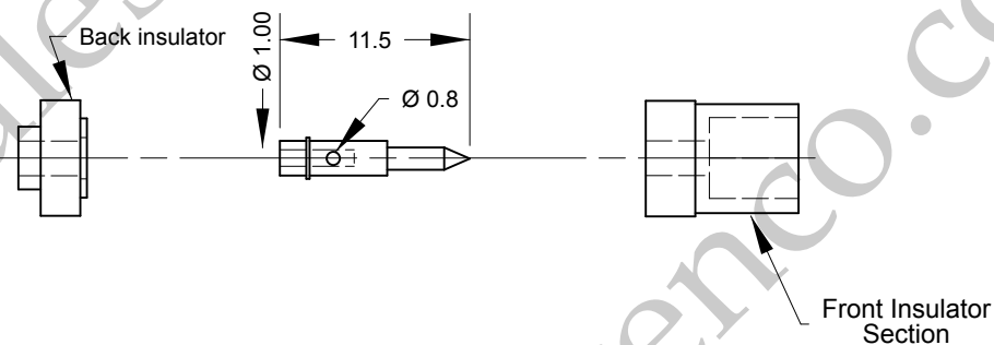
Cable preparation details
