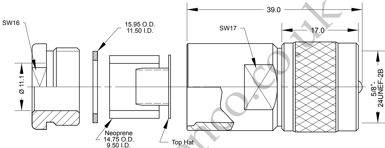
Cable : RG213, RG214 & Equivalents
